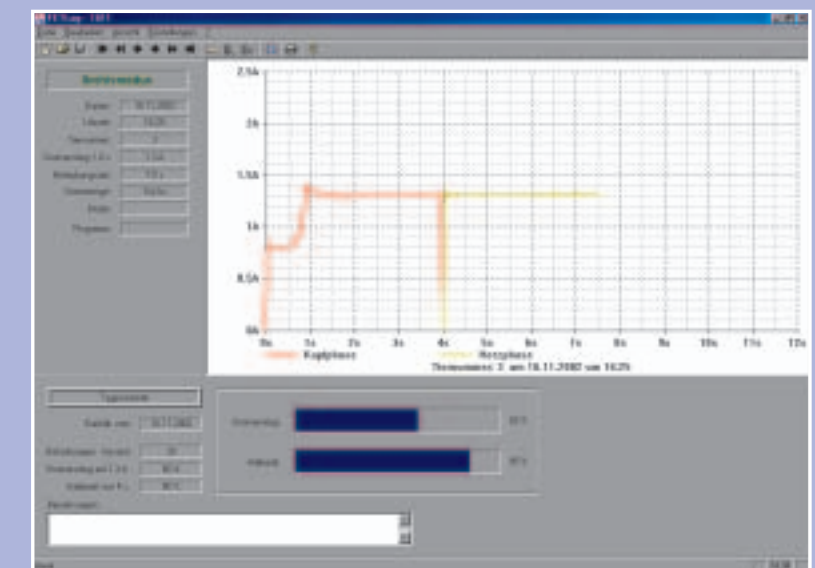
Registering device FBTA and PC for recording of the stunning parameters in accordance with animal protection guidelines and for optimizing the meat quality
